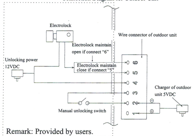
Connection Diagram for Outdoor Unit
